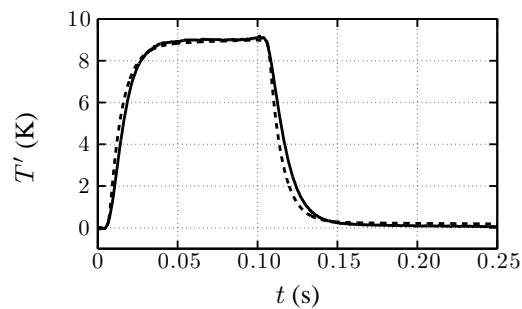
Figure 4 : Time traces of the experimental (—) and numerical (---) temperature downstream of the heating location
