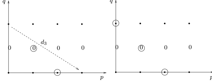
FIGURE 2. Terms E_3^{pq}(\mathcal{X}) and E_4^{pq}(\mathcal{X})
